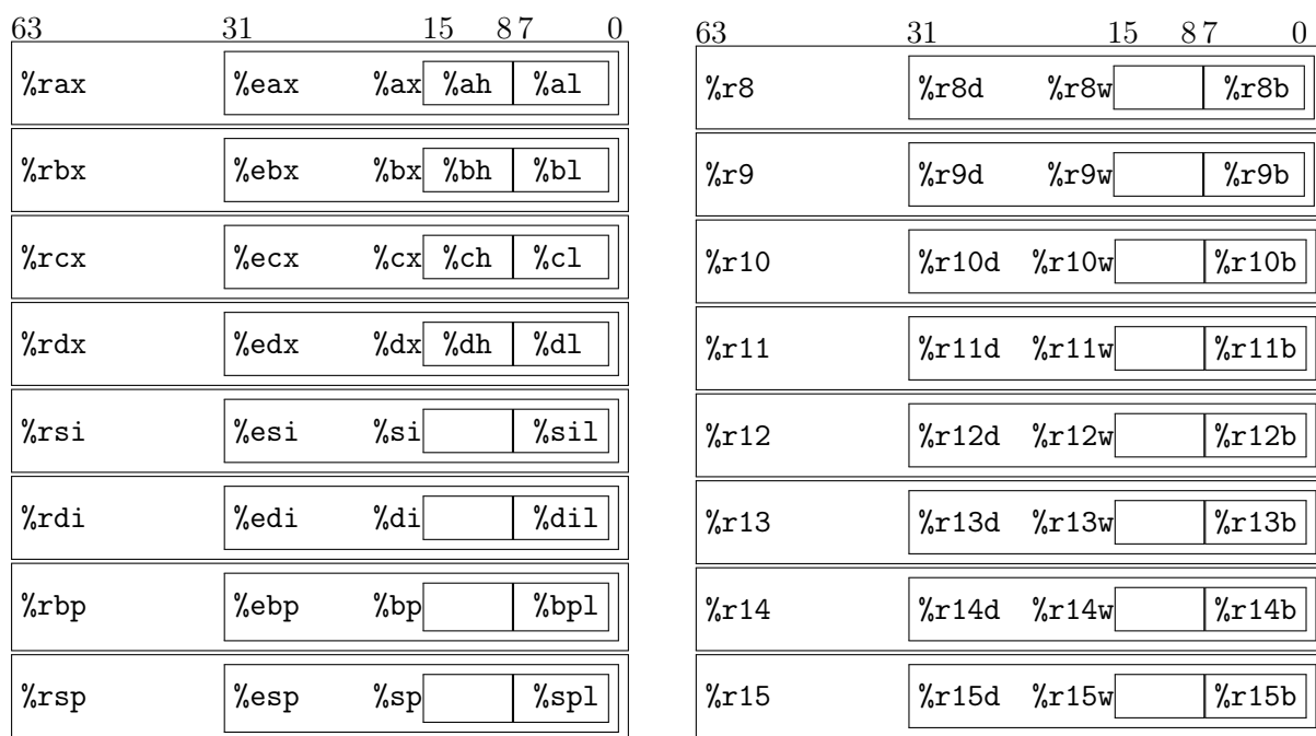
FIGURE 1.1 – Les 16 registres x86-64.
