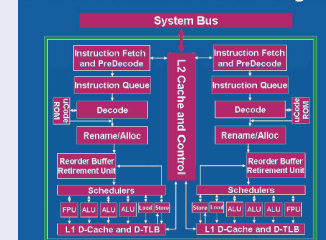
Conroe Processor Block Diagram
